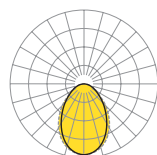
TNEMP/600-1200 LED 7300 lm 840
